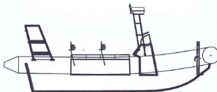
Side Elevation
